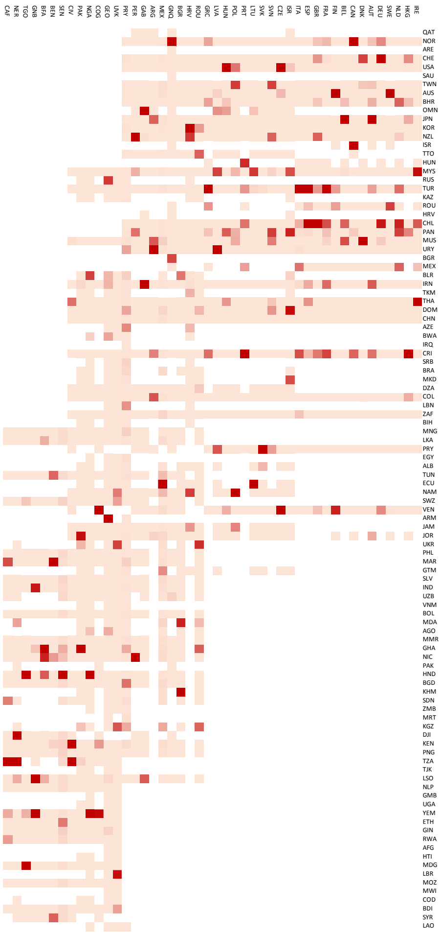
Figure 5: Matrix of Donor Weights in the Baseline SDD Specification
